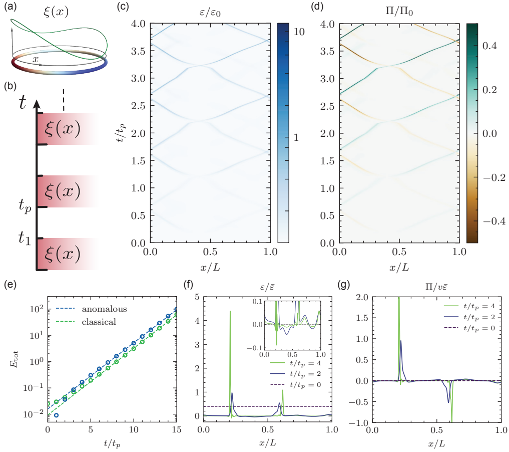
Figure 5: Floquet heating state . (a) and (b) We consider a ring of free relativistic fermions with a spatially modulated velocity \xi(x)v_F = 1 . The modulation \xi(x) is periodic in time with a period t_p = t_1 + t_2 , such that (i) during time t_1 set to the smooth profile shown in (a), and (ii) during time t_2 no modulation is applied and \xi(x) = 1, \forall x . The two times Lt_1/v_F = 0.1 and Lt_2/v_F = 0.45 , are chosen such that the period coincides with the time of flight of particles around the ring: L = v_F t_1 + \tilde{v}_F t_2 where \tilde{v}_F is the averaged effective velocity over the profile \xi(x) . (c) and (d) As a function of time, both the energy density \varepsilon and the momentum \Pi become highly inhomogeneous, and concentrate on a few trajectories. They are represented rescaled by the classical values \varepsilon_0 = v_F \Pi_0 = \gamma T_0^2 . The energy and momentum profiles are represented after two and four periods in panels (f) and (g), illustrating the localization mechanism. (e) Besides being focused spatially, the net energy of the ring E_{\text{tot}} = \int_0^L \varepsilon dx = L\bar{\varepsilon} increases: the Floquet state is heating. This is represented by monitoring the stroboscopic dynamics at times t_n = nt_p of the ring for which E_{\text{tot}} increases exponentially. Remarkably the rate of increase of this energy is not classical: quantum fluctuations, responsible for the trace and gravitational anomaly corrections, have a growing energy. The two focusing trajectories behave as heating black holes: in their neighborhood the energy density becomes negative, as shown in the inset of panel (f). This is an additional manifestation of the effects of quantum fluctuations induced by a local large curvature similar to those in a black-hole atmosphere.
