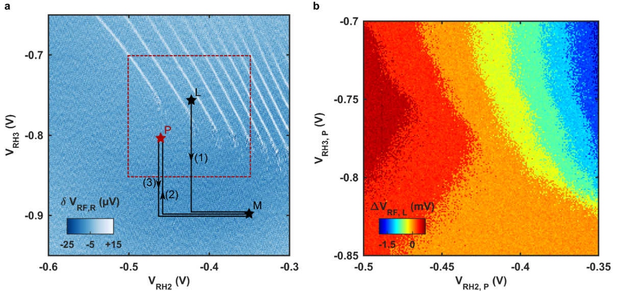
Supplementary Figure 2. Isolated regime. a, Scheme of the pulse sequence. Two electrons are loaded at point L, and the signal is recorded for 5 ms at point M. We then pulse at a point P for 1 ms, and come back to M for another 5 ms measurement. b, Signal difference before and after the pulse, as a function of the position of the point P, each pixel corresponding to a single-shot realization. In the upper part of the figure, the system is connected to the reservoir and the obtained charge states match perfectly the transitions seen in the charge stability diagram. In the lower part of the diagram (orange area), we can keep our two electrons isolated from the reservoir for the duration of the experiment. This ability to turn on and off the coupling to the reservoir is mandatory to avoid accidental charge exchange via the S W potential modulation.
