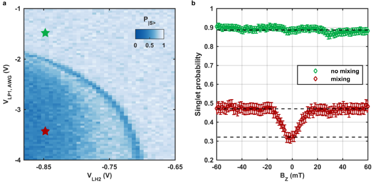
Supplementary Figure 3. Spin initialization and readout fidelity. a , Two-electron spin map on the left double dot. The vertical (resp. horizontal) axis is equivalent to the detuning (resp. the tunnel coupling t ) between the two dots. On the bottom-left part, we see S - T_0 mixing in the (1,1) configuration when the exchange coupling is small. The curved line corresponds to S - T mixing. The two marked positions are used for the spin readout calibration. b , Measured singlet spin probability as a function of the magnetic field, using a 200 ns WG pulse to the two marked positions. In the (2,0) configuration, the singlet spin is always preserved. In the (1,1) configuration, mixing with the |T_0\rangle state occurs at high magnetic field and the expected singlet population is 50 %. For |B_z| < 20 mT, the triplet degeneracy is not lifted and all spin states are mixed, reducing the singlet population to 33 % 30 . From those three asymptotes (dashed black lines) we can extract our spin loading and readout fidelities.
