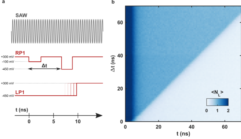
FIG. 3. Controllable injection in moving quantum dots. a , Scheme of the injection timing measurement. Two voltage pulses of a 2.5 ns duration, synchronized with the S W burst, are applied on gate RP1 of the sending dot to trigger the injection of the two electrons into the moving quantum dots. To measure the electron distribution in the moving dots, the reception dot is kept in a configuration where electron catching is unlikely until a positive voltage pulse on LP1 is applied. We take the first electron injection as the reference time t = 0 ns. b , Average charge caught on the reception dot depending on the injection and catching pulse delays. Each pixel is the average of 4000 single-shot realizations. The vertical and diagonal boundaries correspond to the arrival time of the first and second electron, respectively. The vertical boundary begins at t_s = 2.1 ns as a consequence of the time of flight at the S W velocity of the first electron between the two static dots. Moreover, the clean and sharp diagonal boundary with unity slope confirm our ability to control the separation of two electrons by up to 70 ns with a nanosecond resolution, using a double WG voltage pulse. The precision of the sending is measured close to a nanosecond and fixed by the rise time of the WG.
