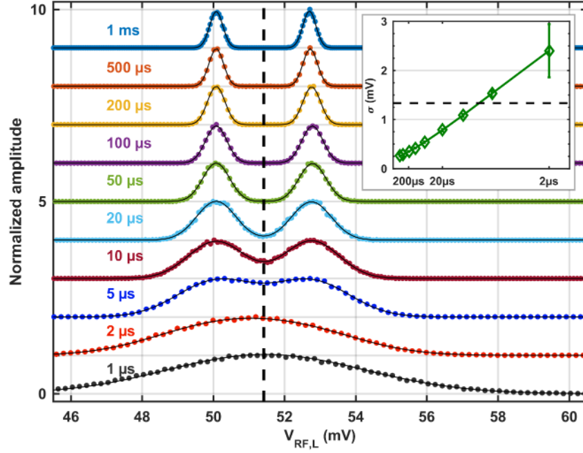
Supplementary Figure 1. Charge sensing and measurement bandwidth. Histogram of the signal obtained by loading successively 1 or 2 electrons in the left quantum dot as a function of the integration time. The curves have been normalized and offset for clarity, and fitted with a double Gaussian distribution (solid black line). The dashed black line represents the threshold used for charge assignment, positioned in the middle of the two peaks. Inset, Mean standard deviation of the two electron Gaussian peaks as a function of 1/\sqrt{t_{meas}} . The noise is inversely proportional to the square root of the integration time, and overcomes the threshold for t_{meas} < 6 \mu s (SNR= 1). For t_{meas} > 30 \mu s, the charge readout fidelity is greater than 95 %.
